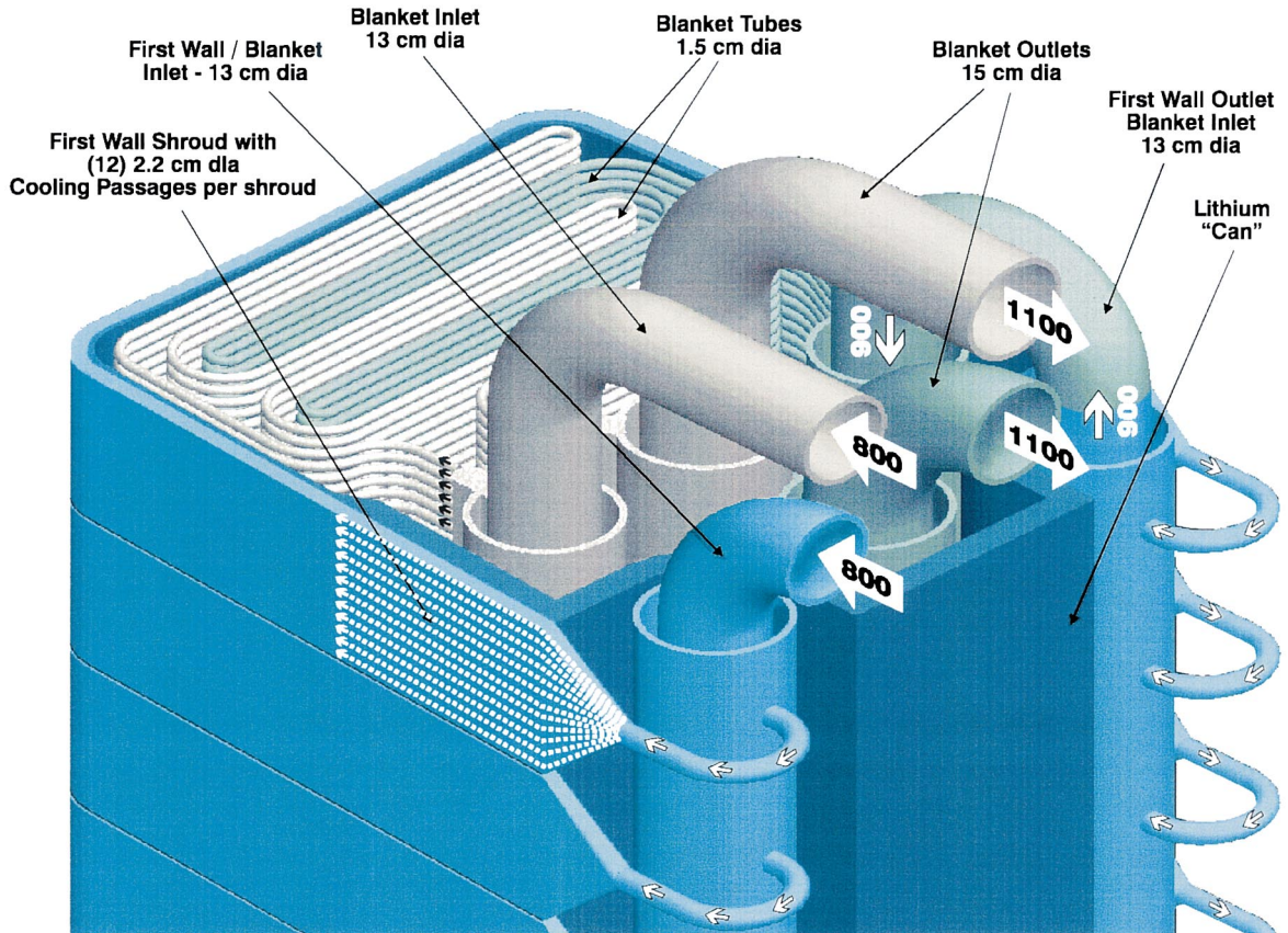
Fig. 35. Helium-cooled first wall and divertor design module.
