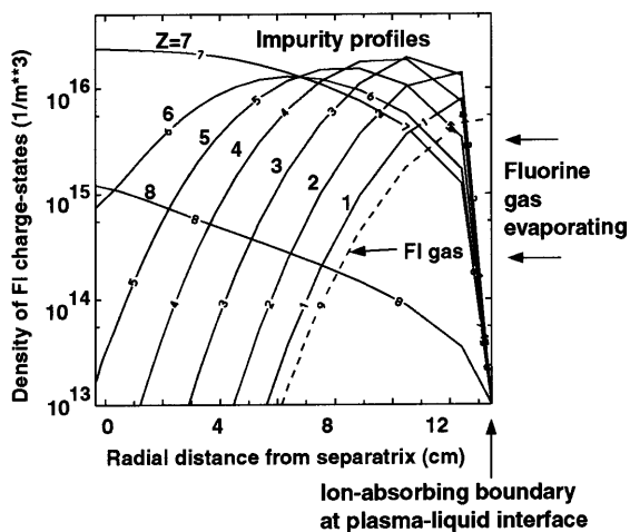
Fig. 31. Density of fluorine charge-states at the outer midplane for a gas wall flux of 8 \times 10^{18} \text{ m}^{-2}\text{s}^{-1} in the standard tokamak geometry.
