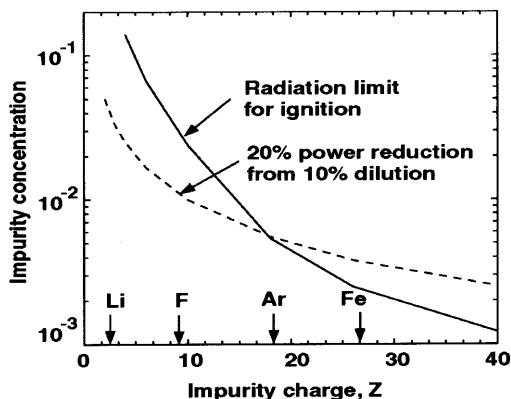
Fig. 30. Impurity concentration limits for different impurities due to radiation loss in a tokamak (solid line) and due to simple fuel dilution (dashed line).
