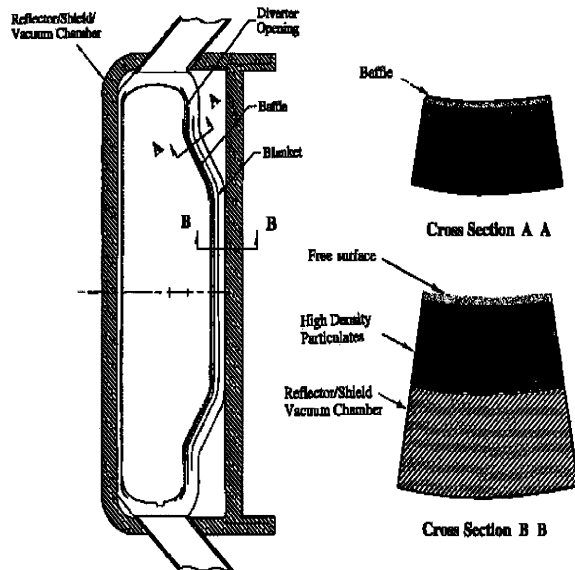
Fig. 39. APPLE configuration using baffles.
