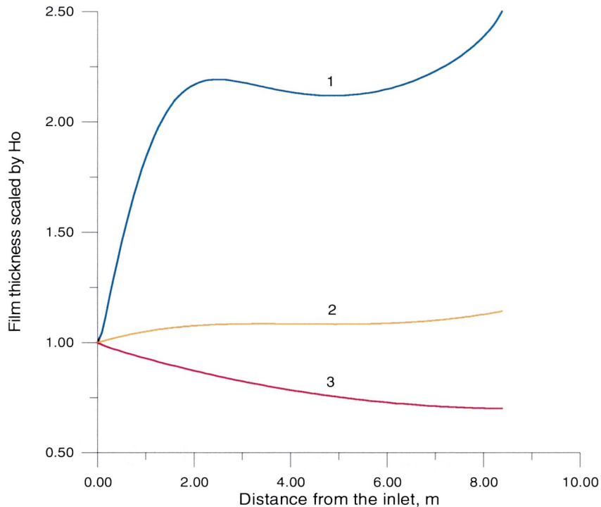
Fig. 25. Surface height predictions for Flibe with various models: Line 1: \kappa - \varepsilon , 2: Darcy Weisbach friction factor = 0.025, and 3: laminar.
