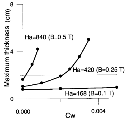
Fig. 28. Influence of the radial magnetic field and the wall conductance ratio on the maximum thickness of the lithium layer (for axi-symmetric case, C_w = \infty ).
