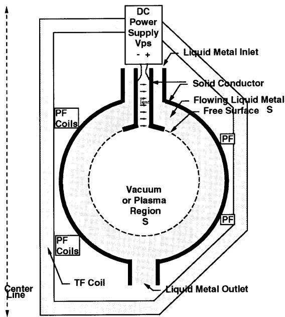
Fig. 29. Electromagnetic restraint (EMR) lithium blanket concept.
