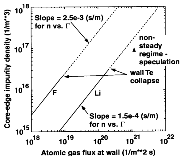
Fig. 32. Comparison of fluorine and lithium densities at the core boundary for different gas fluxes at the first wall. The dotted lines are extrapolations owing to non-steady solutions which arise with a collapse of the electron temperature just in front of the wall for larger gas fluxes.
