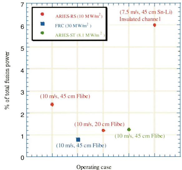
Fig. 14. The pumping power as a fraction of fusion power for various cases of liquid wall thickness and confinement configurations. Note that the pumping power is scaled from that of the HYLIFE-II design, taking into account the 50% head recovery. The effect of MHD drag will increase the calculated pumping power of a Sn–Li flowing liquid wall.
