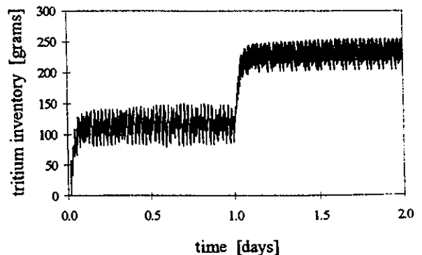
Figure 7: Dynamic Tritium Inventory in the ISS
