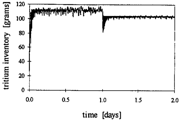
Figure 8: Dynamic Tritium Inventory in Fuel Management
