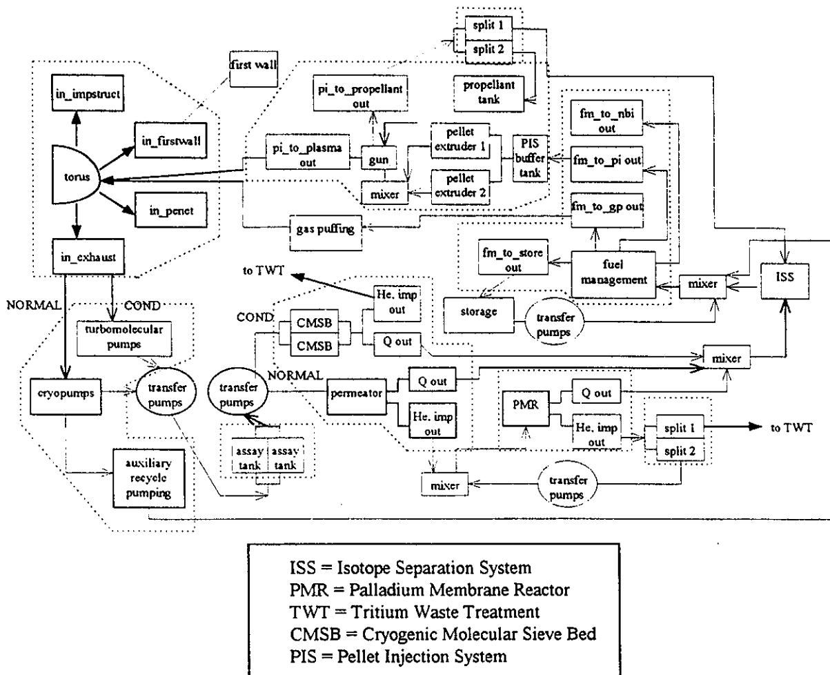
Figure 1: Proposed ITER Tritium Processing System Flowsheet
