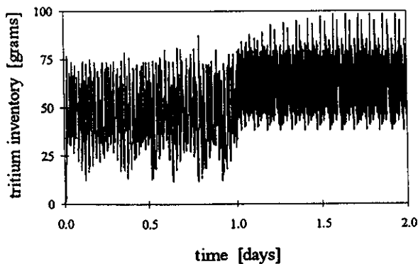
Figure 5: Dynamic Tritium Inventory in Assaying Tank System
