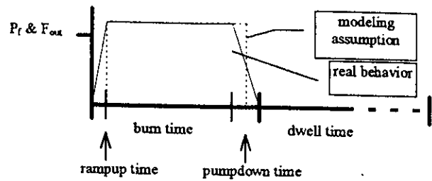
Figure 2: Power and Fuel Outflow Cyclic History
