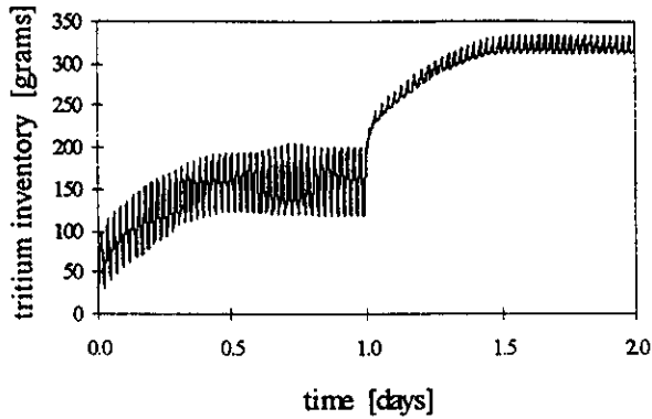
Figure 4: Dynamic Tritium Inventory in Cryopumps
