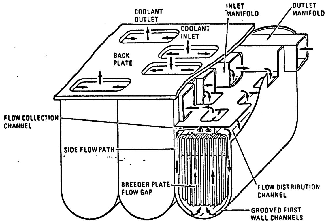
Helium coolant flow path in the blanket.
