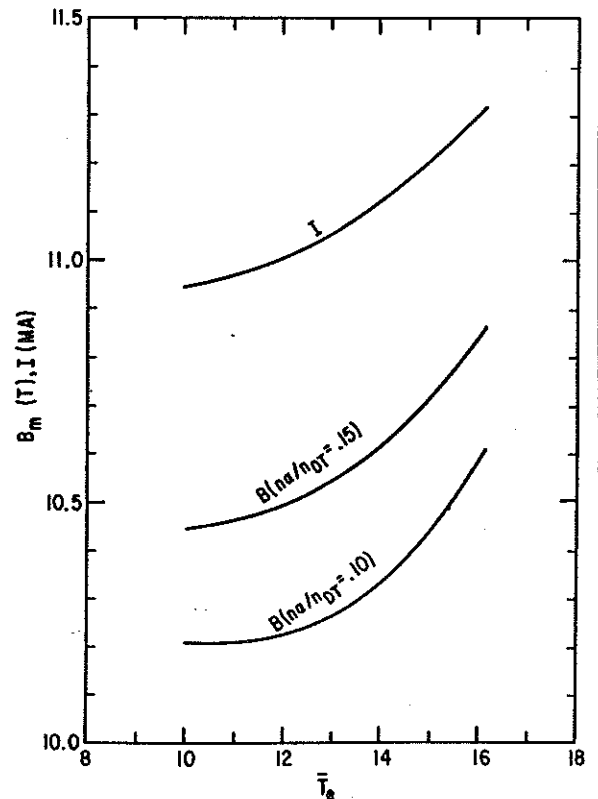
Fig. 5. Variation of the maximum magnetic field and plasma current with the average electron temperature, T_e . ( P_f = 3200 MW, \kappa = 1.6 , A = 3.6 , R = 7 m, \beta_t = 0.067 , \Delta_{BS}^1 = 1.2 m, \Delta_v = 0.1 m.)
