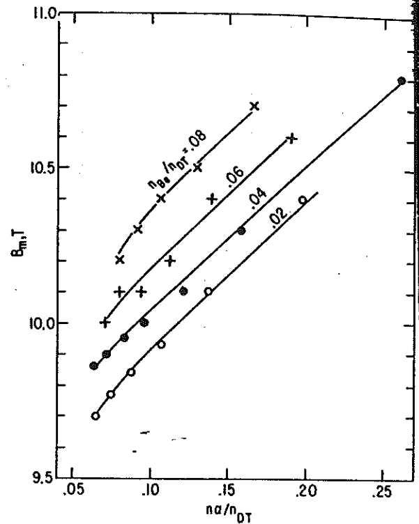
Fig. 4. Variation of the maximum magnetic field with the alpha-particle concentration, n_\alpha/n_{DT} , and other impurity concentration, n_{Be}/n_{DT} . ( P_f = 3200 MW, P_{nw} = 3.5 MW/m 2 , \kappa = 1.6 , A = 3.6 , \beta_t = 0.067 , T_i \sim T_e = 14 keV, \Delta_{BS}^1 = 1.2 m, \Delta_v = 0.1 m, R = 7 m.)
