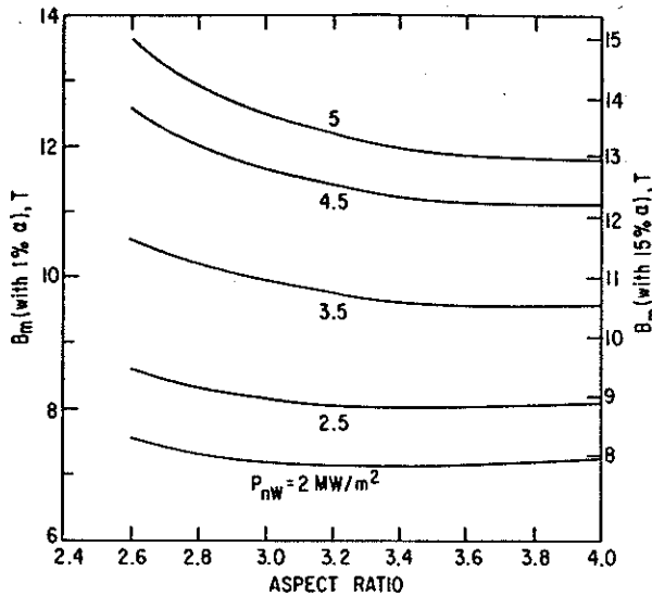
Fig. 3. B_m as a function of A at several values of P_{nw} . The LHS scale is for n_\alpha/n_{DT} = 0.01 and the RHS scale is for n_\alpha/n_{DT} = 0.15 . ( P_f = 3200 MW, \beta_t = 0.24/A , \Delta_{BS}^1 = 1.2 m, \Delta_v = 0.1 m, \bar{T} = 8 keV, \kappa = 1.6 .)
