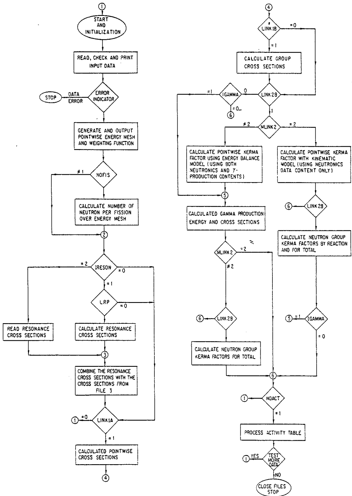
Fig. 1. A flow diagram for MACK-IV.
