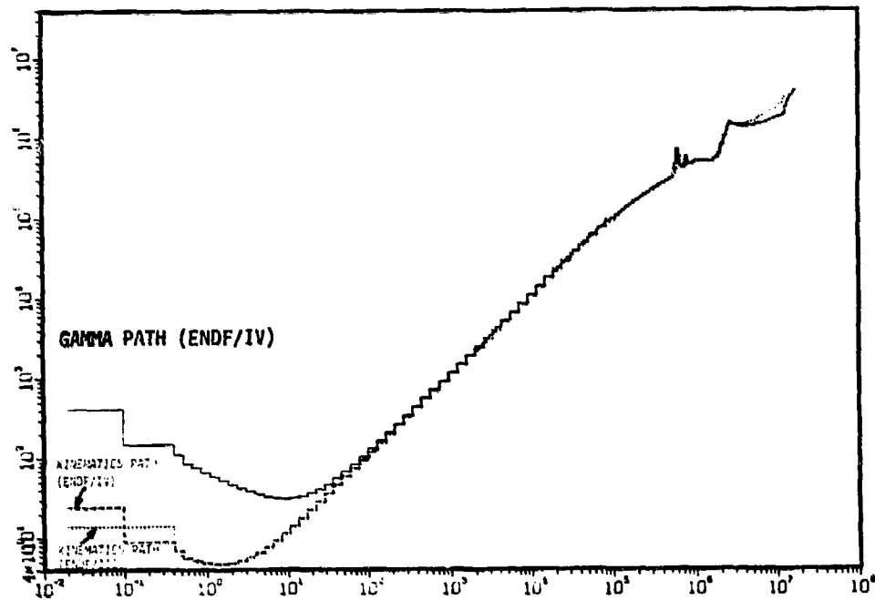
FIGURE 2. Neutron kerma factors for beryllium.
