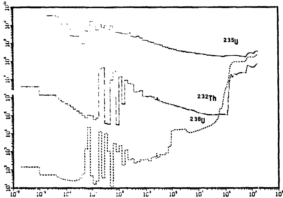
FIGURE 3. Neutron kerma factors for 232 Th, 235 U, and 238 U.
