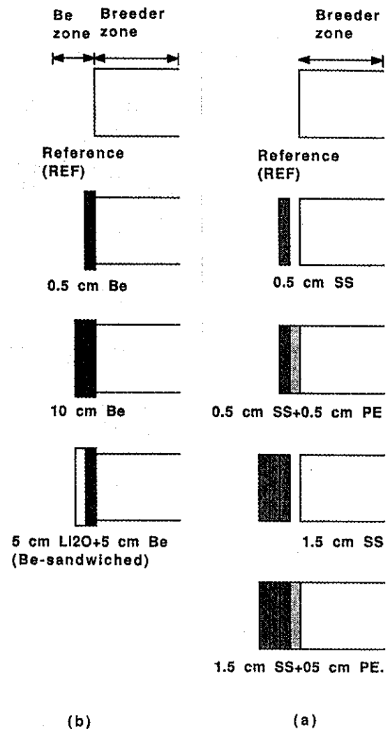
Fig. 1. Arrangements for (a) the first-wall experiments (WFW) and (b) the beryllium experiments (WBE) of Phase I.
