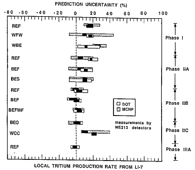
Fig. 8. The prediction uncertainty (%) for T_7 , \bar{X}_r , based on the DOT and MCNP calculations (NE213 measurements).
