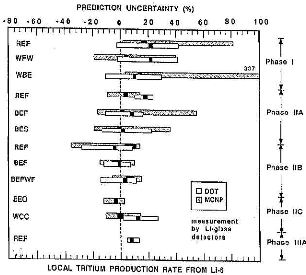
Fig. 7. The prediction uncertainty (%) for T_6 , \bar{X}_r , based on the DOT and MCNP calculations (Li-glass measurements).
