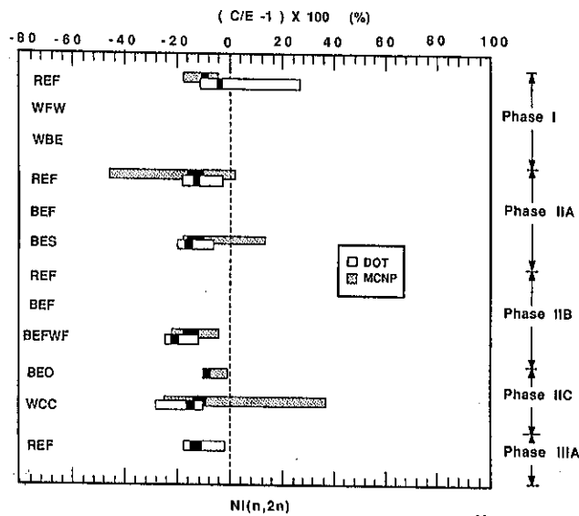
Fig. 10. The prediction uncertainty (%) for the ^{58}\text{Ni}(n, 2n) reactions.
