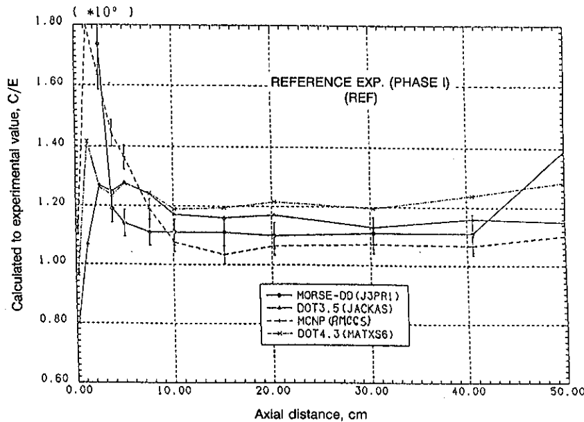
Fig. 5. The C/E values for T_6 in the reference experiment of Phase I (Li-glass measurements).
